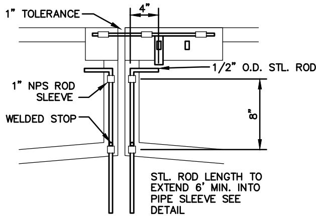
GATE ANCHOR ROD DETAIL (CLOSED)
