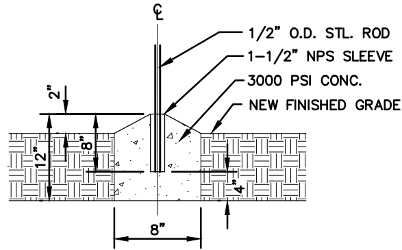
GATE ANCHOR SLEEVE DETAIL (OPEN POSITION)
